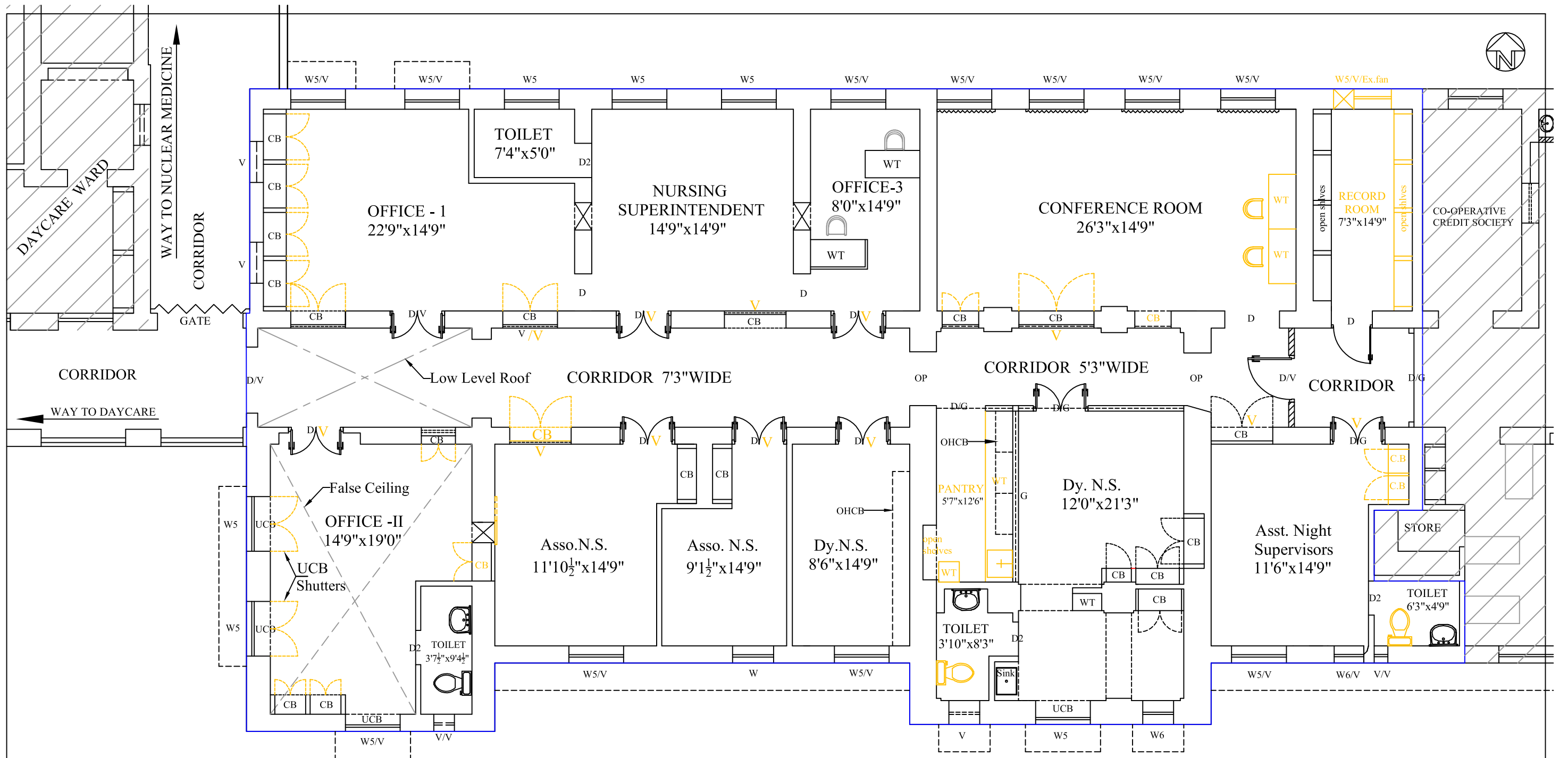
FIRST FLOOR PLAN - NURSING SERVICE OFFICE
